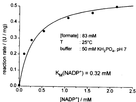
Figure 3: Reaction rate of the new NADP(H) dependent FDH as a function of the NADP + -concentration: measured points and optimized kinetic curve resulting in a K_M for NADP + of 0.32 mM.
